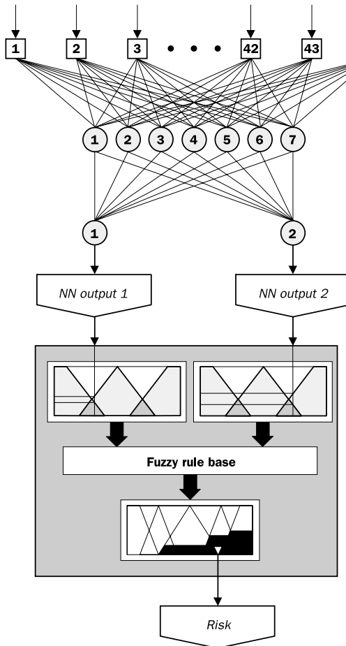
Figure 9.37 Hierarchical structure of the neuro-fuzzy system for risk assessment of the cardiac disease
