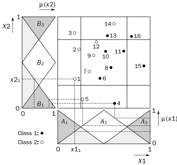
Figure 8.19 Fuzzy partition by a 3 × 3 fuzzy grid
